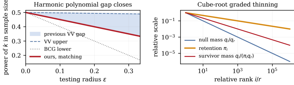
Figure 1: Left: for the harmonic null at fixed \epsilon , previous upper and lower bounds leave a polynomial range. Our matching rate lies on the sharp lower exponent and determines the missing logarithmic factor. Right: the hard prior retains rank i with cube-root probability and inflates survivors, spreading its second-moment cost across the tail.
