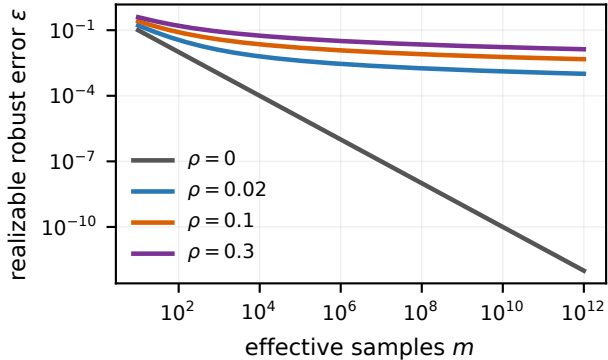
Exact realizable learning curves
