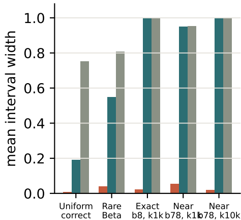
(b) Synthetic width
