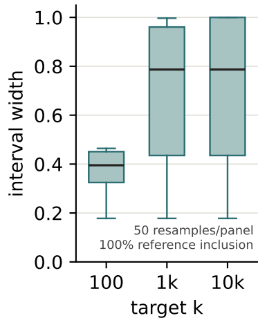
(c) 22 public panels
