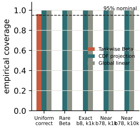
(a) Synthetic coverage
