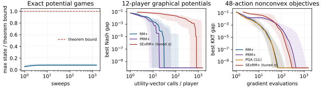
Figure 1: Mechanism and frontier baselines. Left: regret states remain below the theorem’s uniform bound. Middle: alternating methods on graphical exact-potential games. Right: simplex optimization, with PGA given 1/L . SExRM+ is favorably tuned in hindsight from the disclosed grid. Horizontal axes normalize oracle calls. Values at machine zero are displayed at 10^{-10} .
