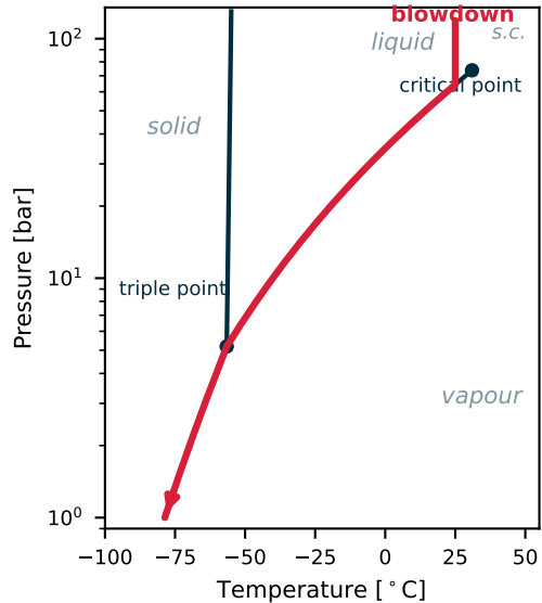
CO 2 phase diagram
