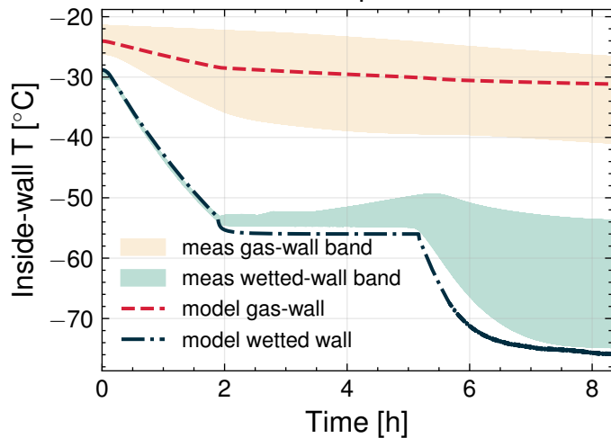
Wall temperature
