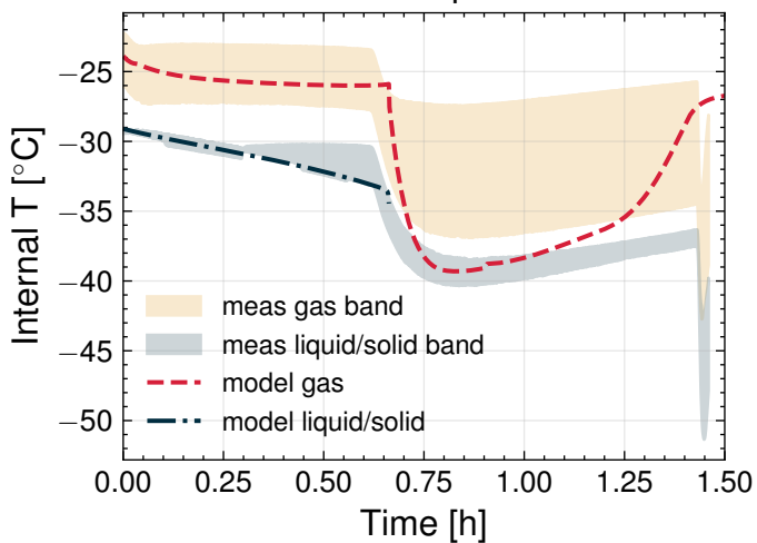
Internal temperature
