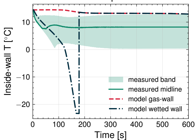
Wall temperature
