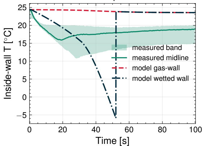
Wall temperature
