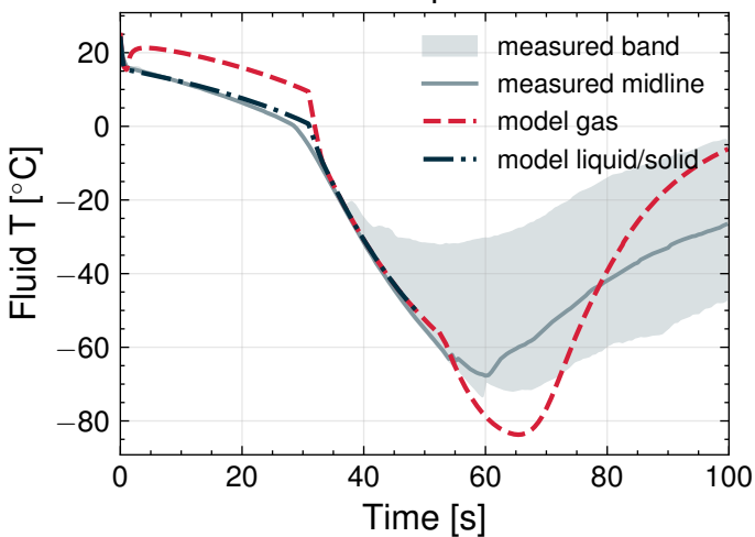
Fluid temperature
