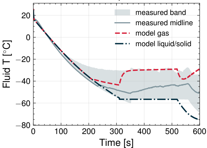
Fluid temperature
