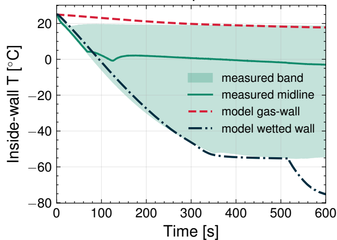
Wall temperature
