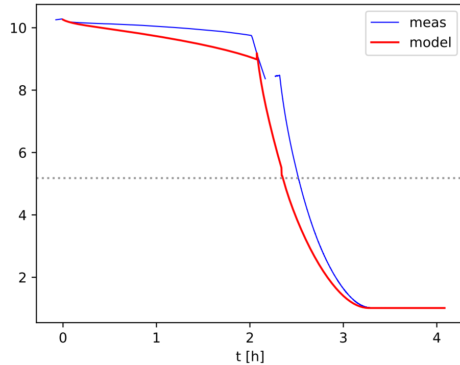
T10 liquid - Pressure [bar]
