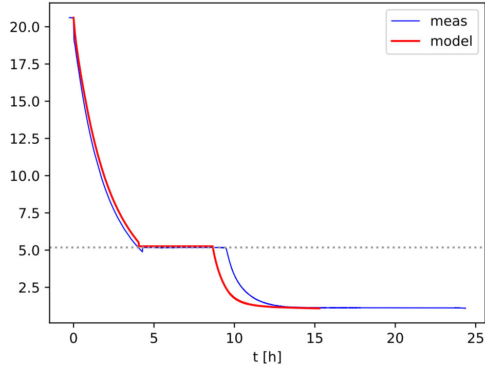
T5 gas - Pressure [bar]
