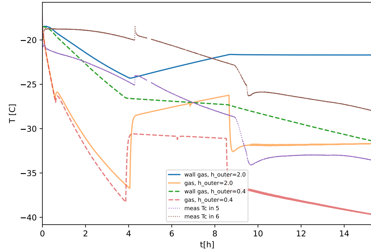
T5 gas + gas-wall temp: h_outer 2 vs 0.4
