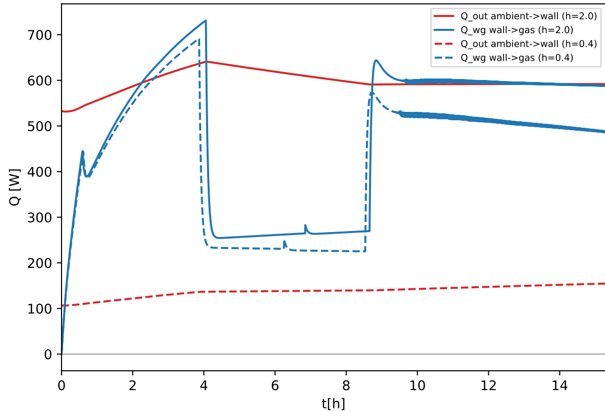
Gas-wall heat terms
