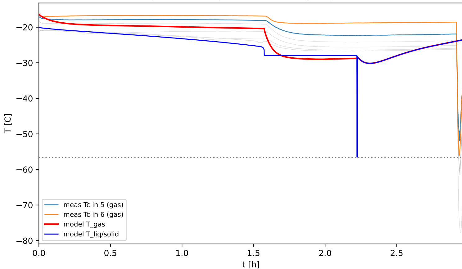
Test 6 (liquid) - model gas vs measured gas-space sensors
