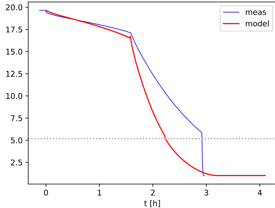
T6 liquid - Pressure [bar]
