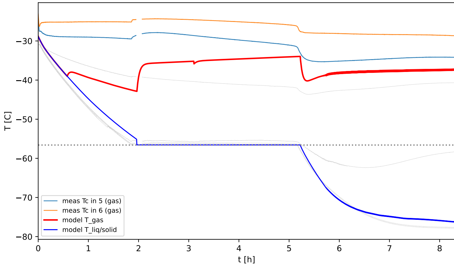
Test 7 (gas) - model gas vs measured gas-space sensors
