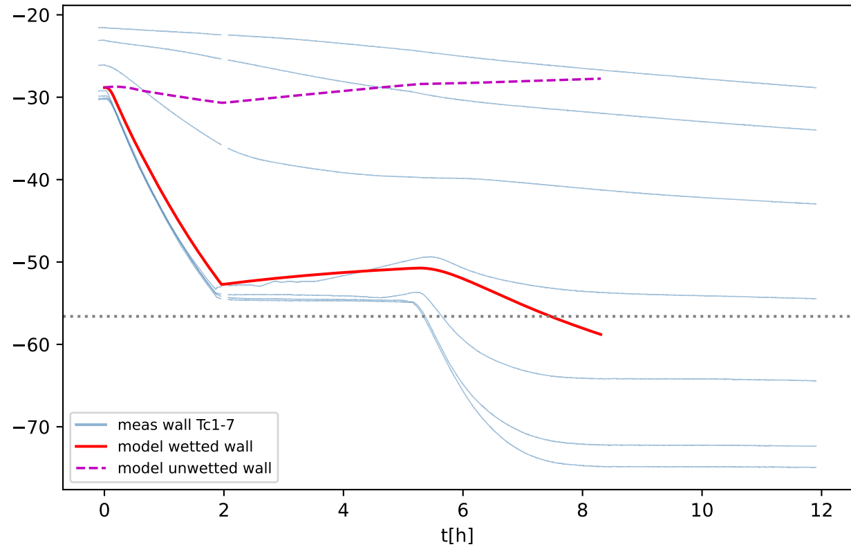
Wall temperature [C]
