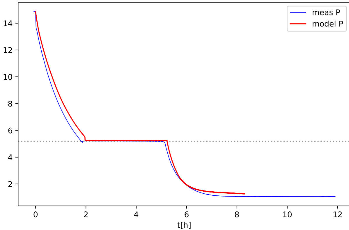
T7 gas Pressure [bar]
