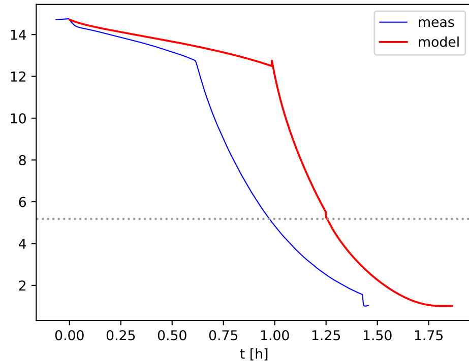
T8 liquid - Pressure [bar]
