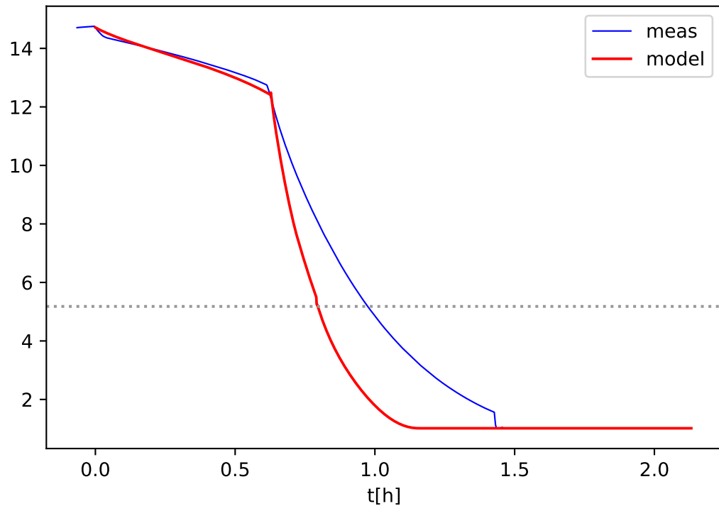
T8 6mm Pressure [bar]
