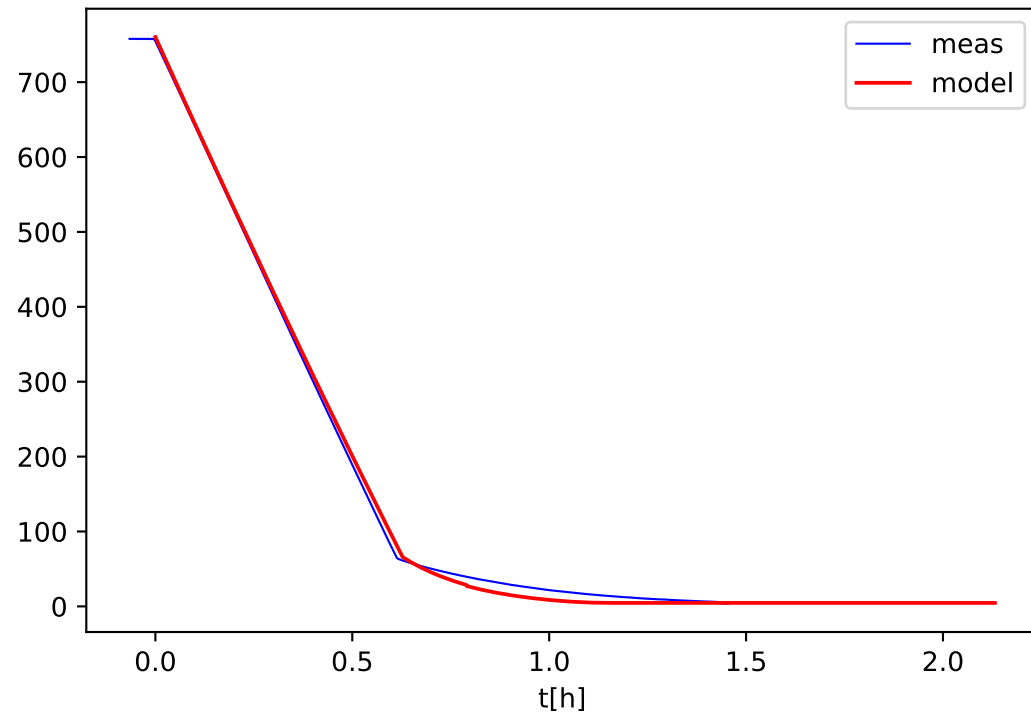
Inventory mass [kg]
