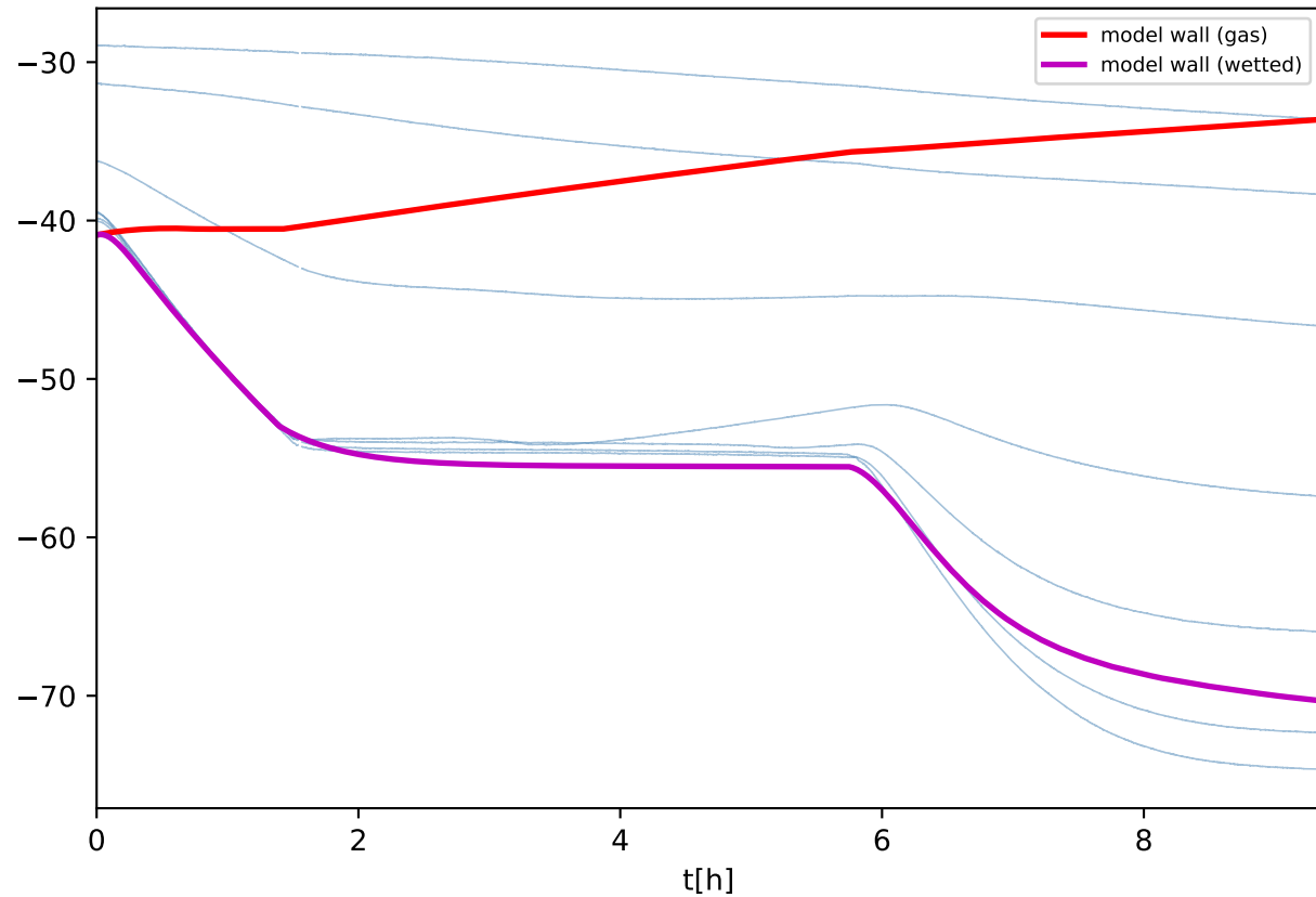
T9 inside-wall temp [C] (all 7 + model)
