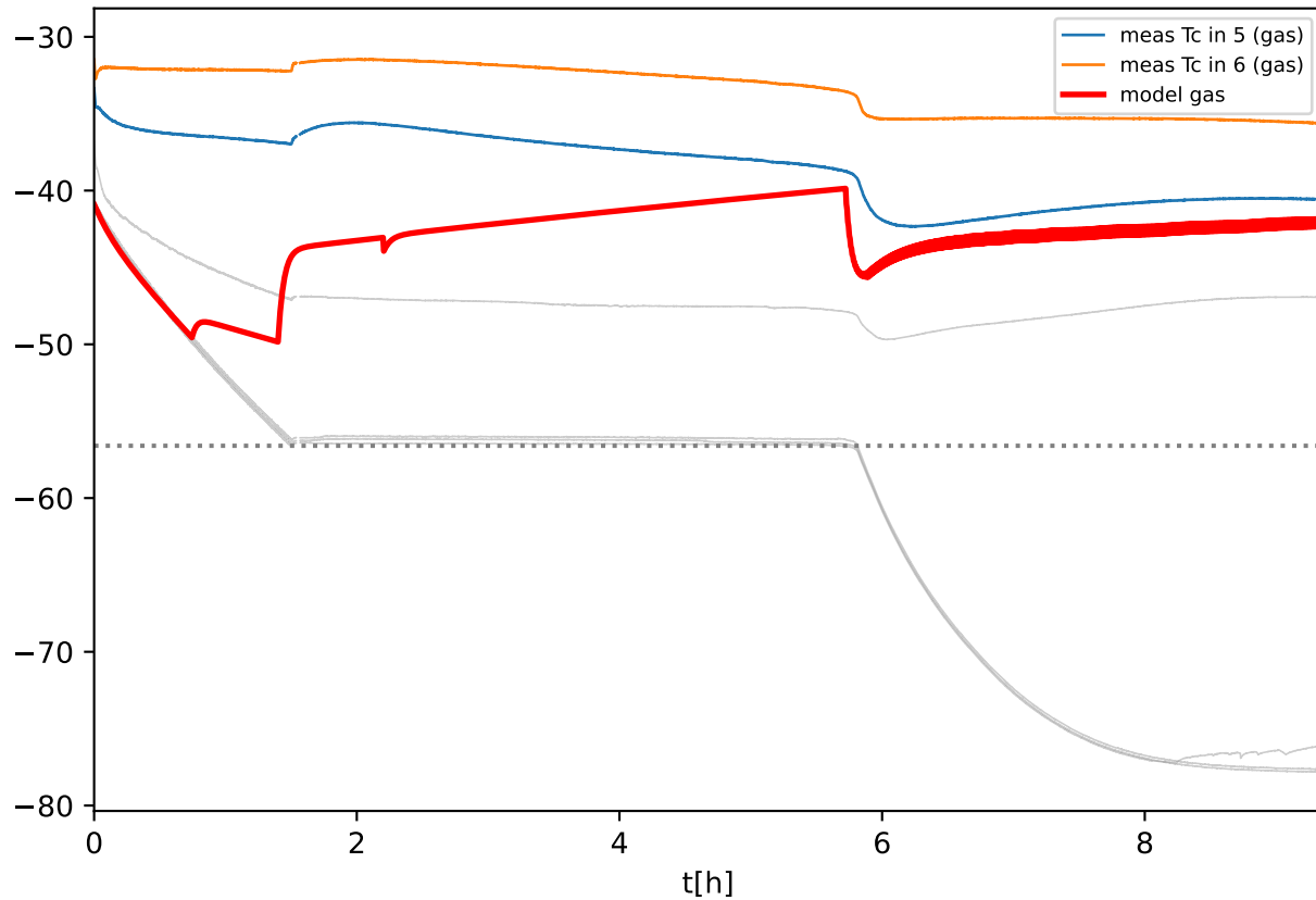
T9 internal/gas temp [C]
