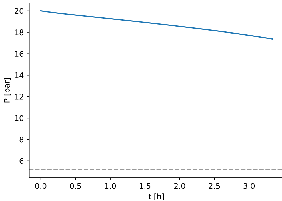
CARDICE Batch 6 — liquid release (current model)
