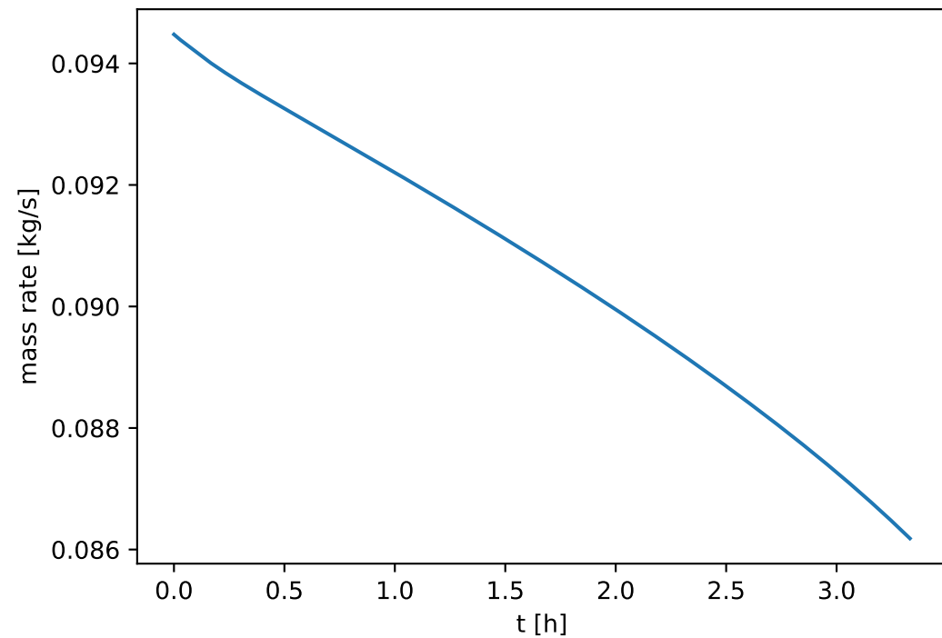
CARDICE Batch 6 — liquid release (current model)
