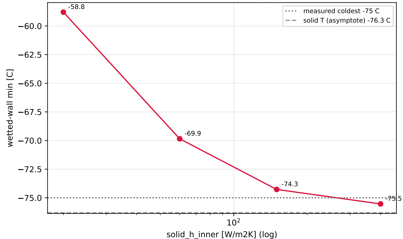
Wetted-wall min vs solid_h_inner
