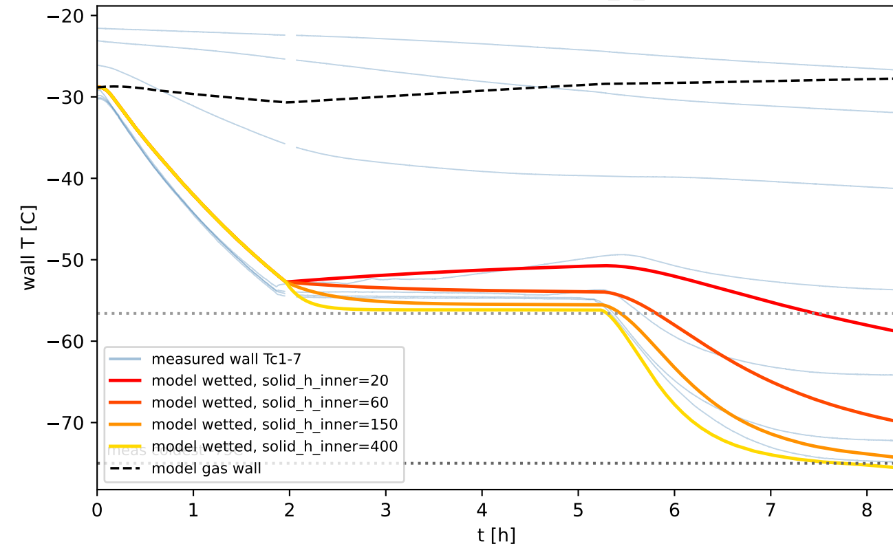
T7 wetted-wall trace vs solid_h_inner
