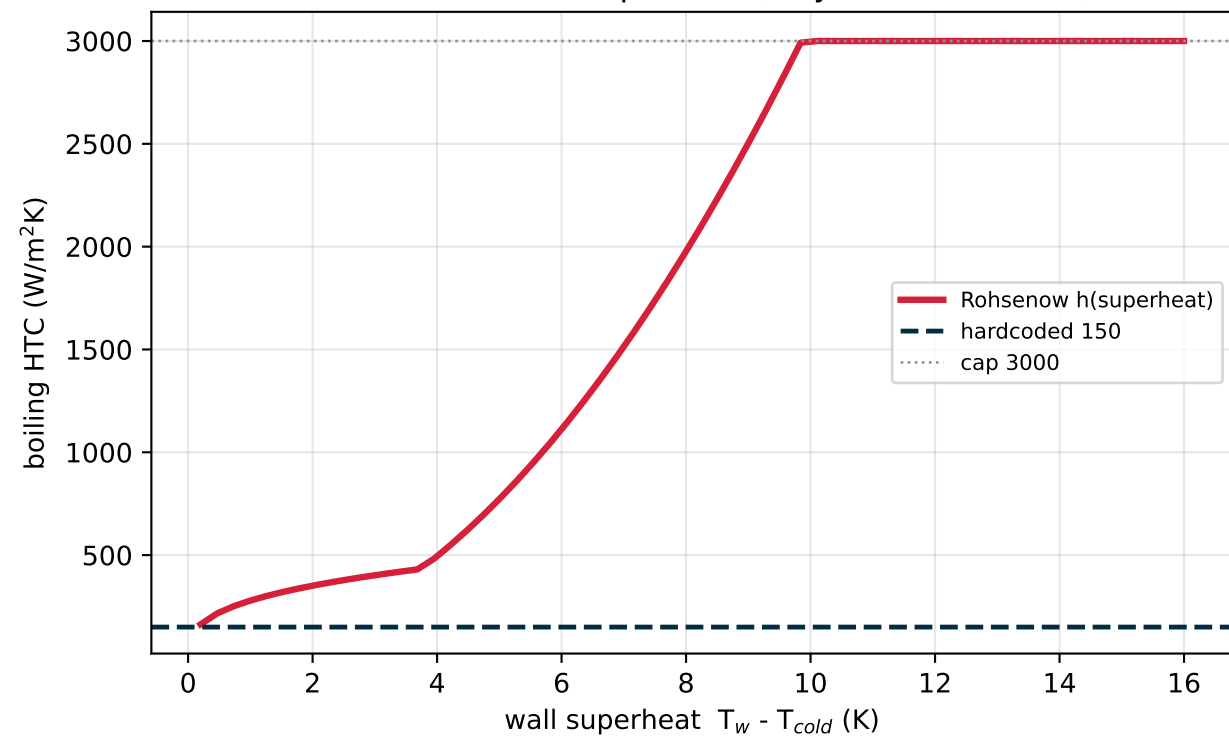
Rohsenow HTC vs superheat (why it matches 150)
