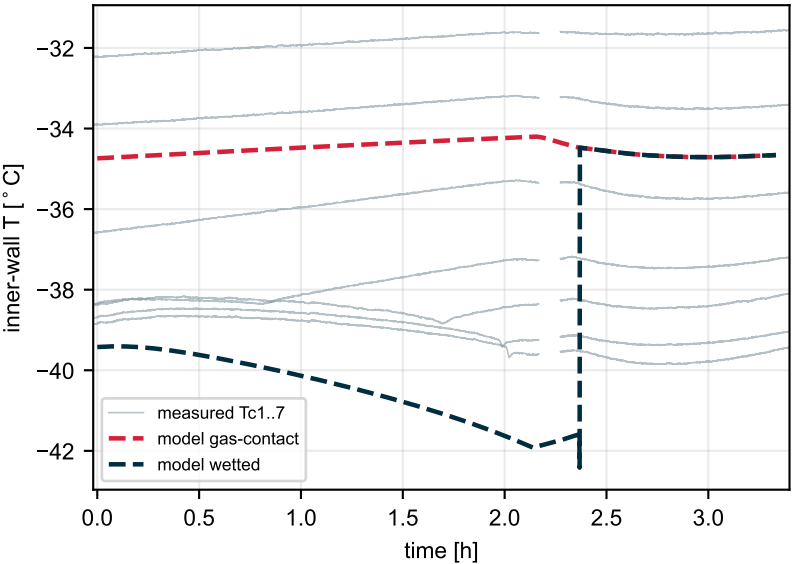
Inner-wall temperature
