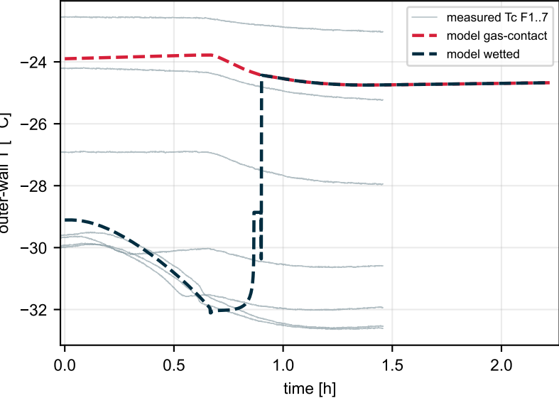
Outer-wall temperature
