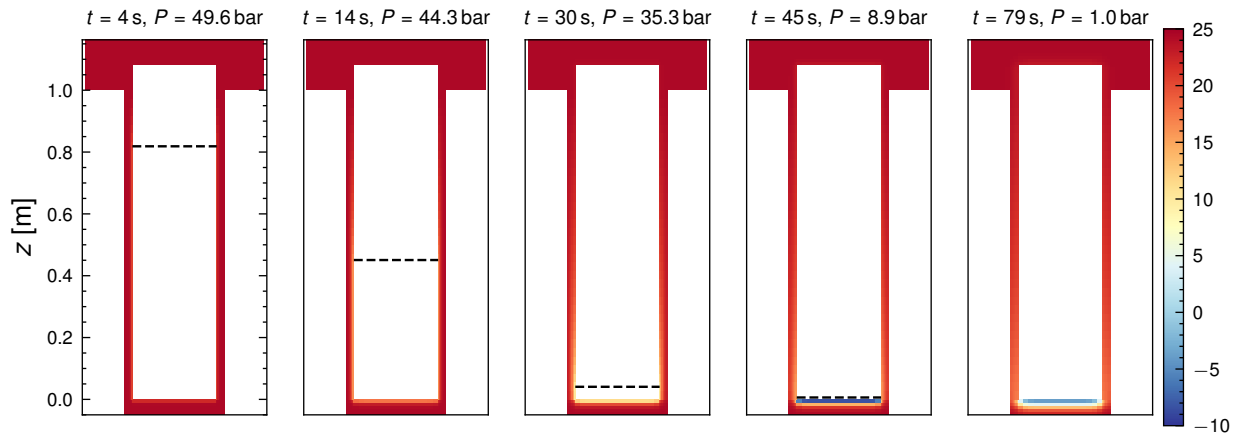
Exp53 (riser / liquid)
