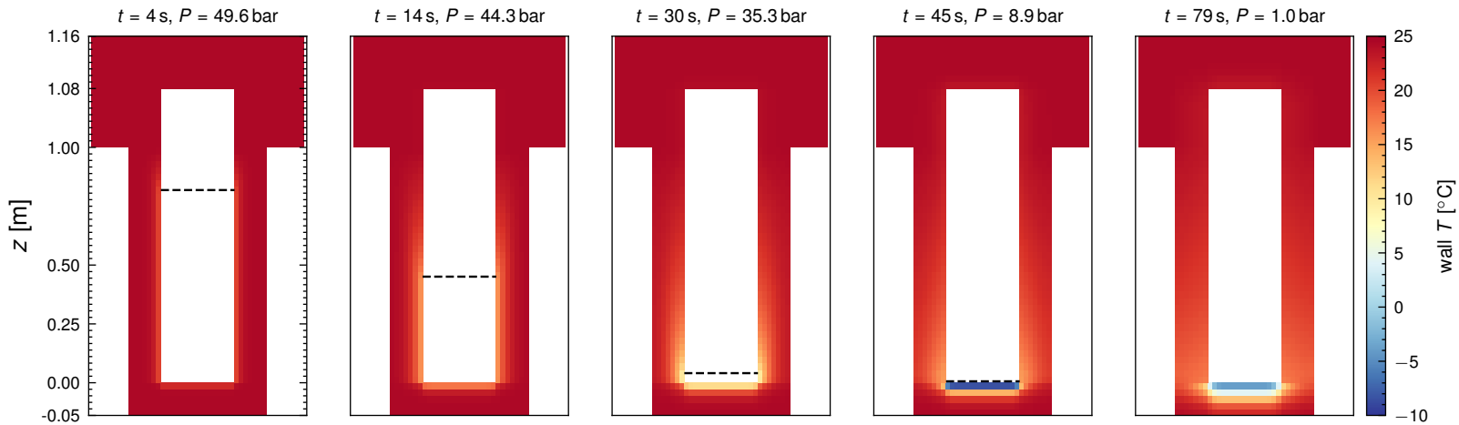
Exp53 (riser / liquid)
