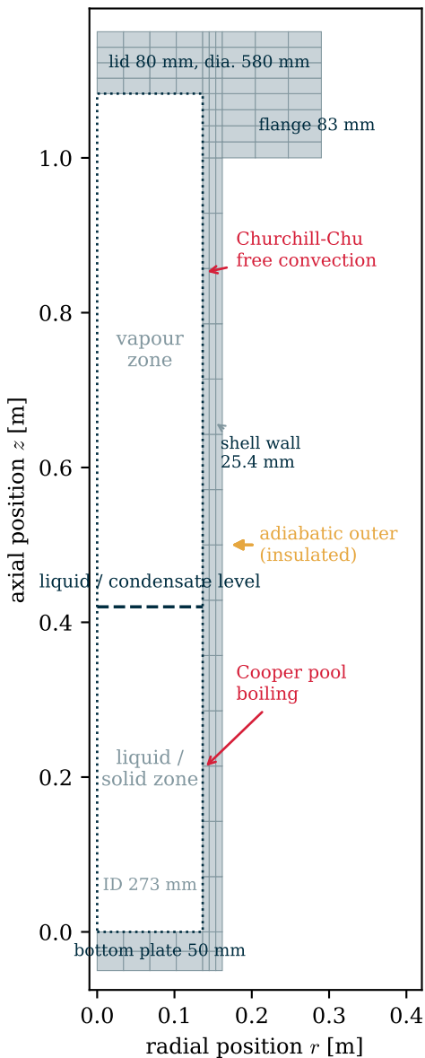
(a) axisymmetric domain and FV grid
