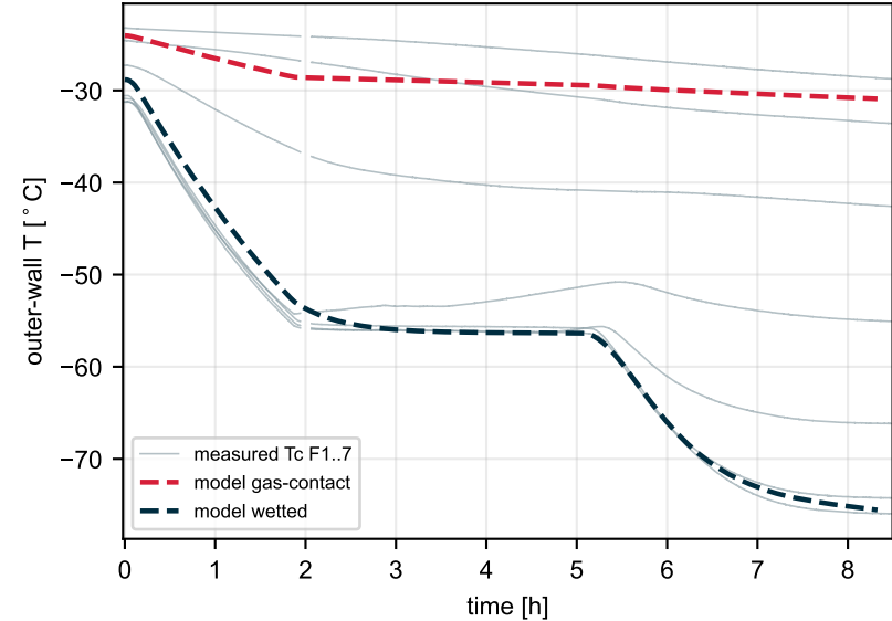
Outer-wall temperature
