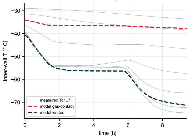
Inner-wall temperature
