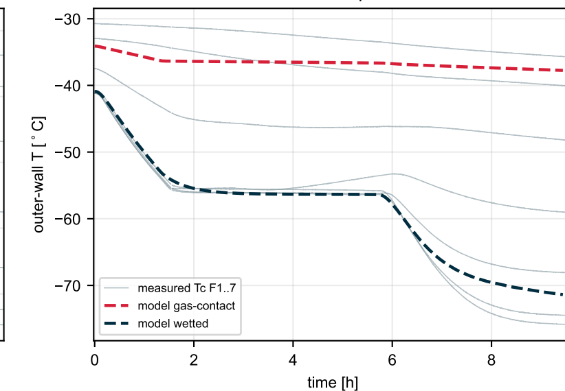
Outer-wall temperature
