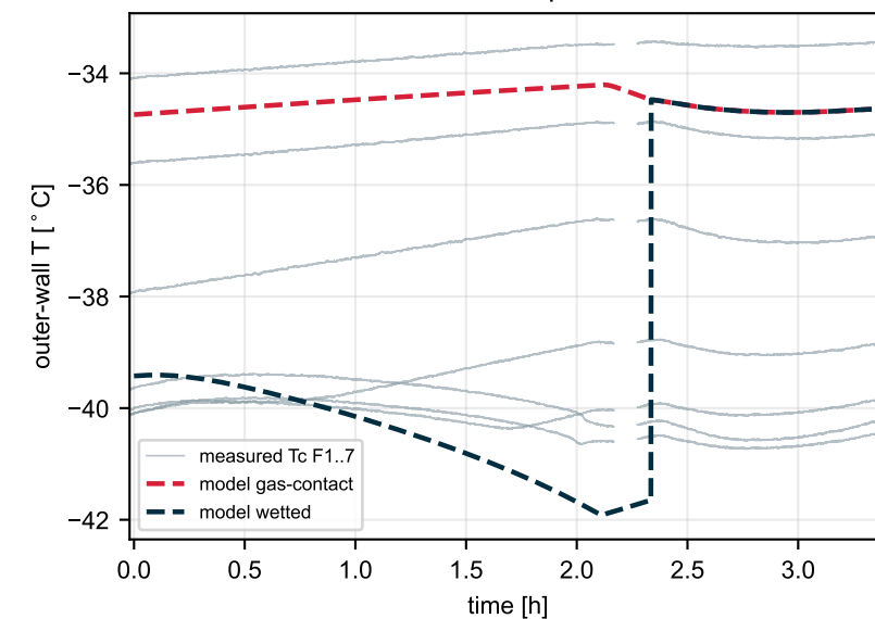
Outer-wall temperature
