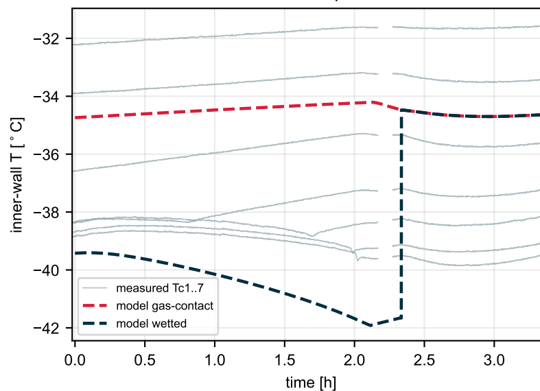
Inner-wall temperature
