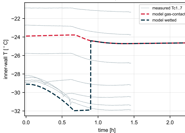
Inner-wall temperature
