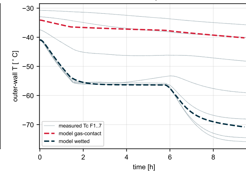
Outer-wall temperature
