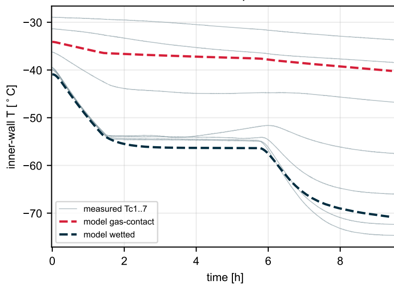
Inner-wall temperature
