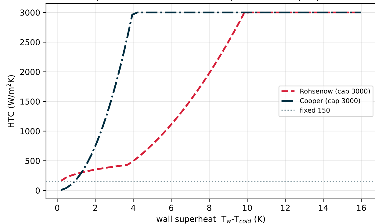
Cooper vs Rohsenow HTC vs superheat (at triple point)
