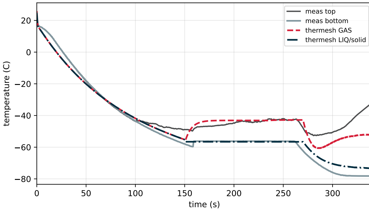
Gas/liquid split (thermesh)
