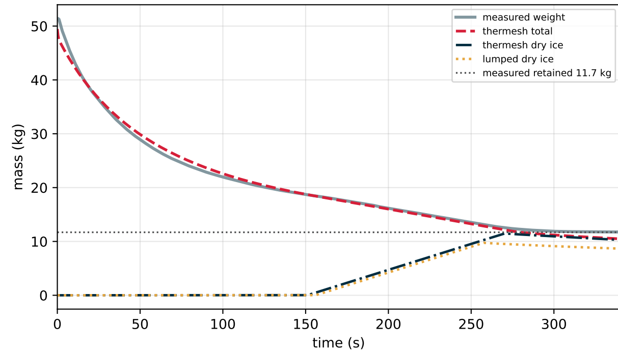
Retained dry ice: thermesh vs lumped vs measured
