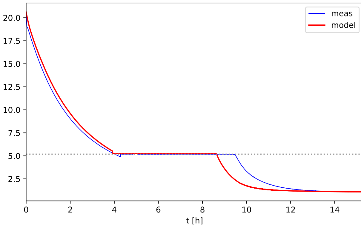
CARDICE Test 5 (gas) - model vs 1 Hz data (all sensors)
