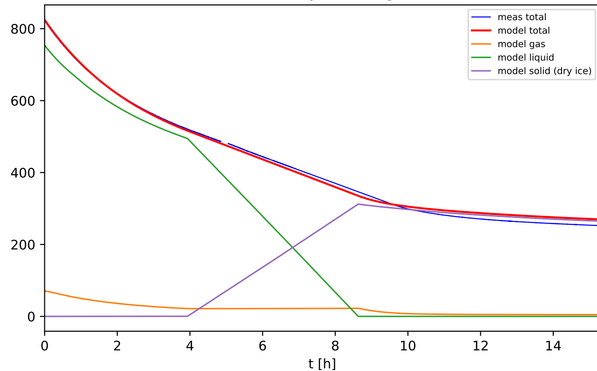
CARDICE Test 5 (gas) - model vs 1 Hz data (all sensors)
