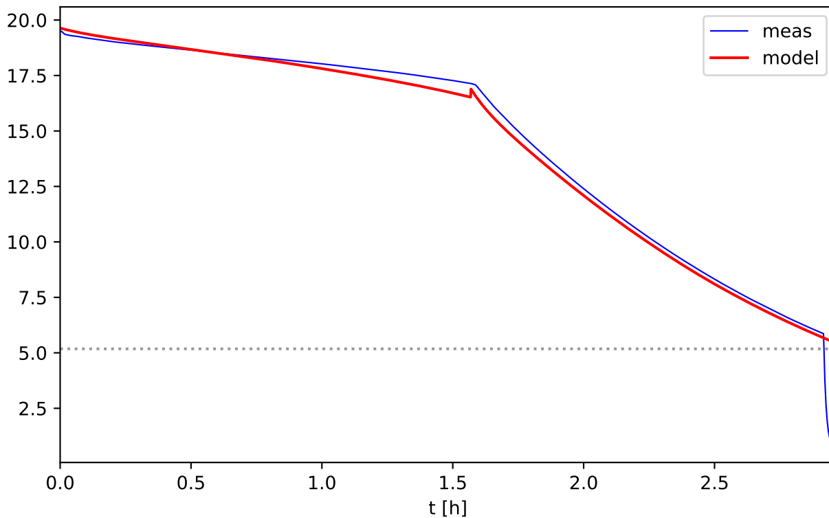
CARDICE Test 6 (liquid) - model vs 1 Hz data (all sensors)
