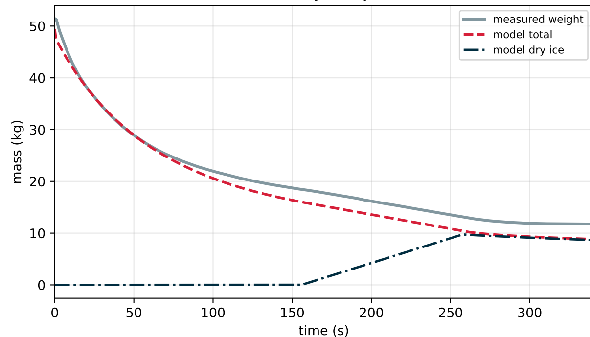
Discharge rate
