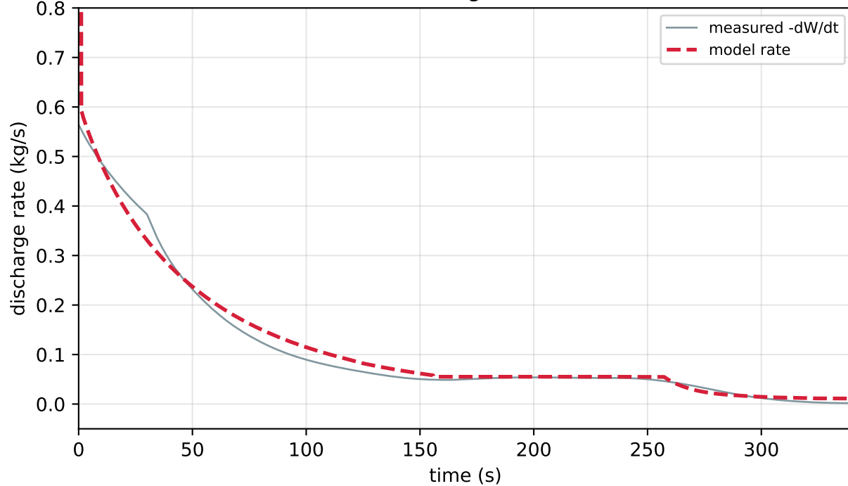
Discharge rate
