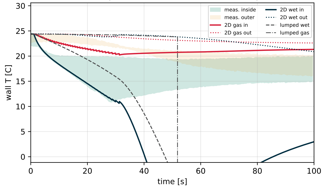
Wall temperature (2D inner/outer vs lumped)
