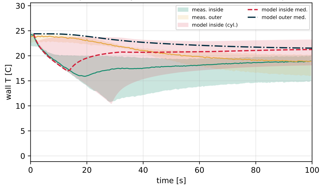
Wall temperature (cylinder inner/outer vs thermocouples)
