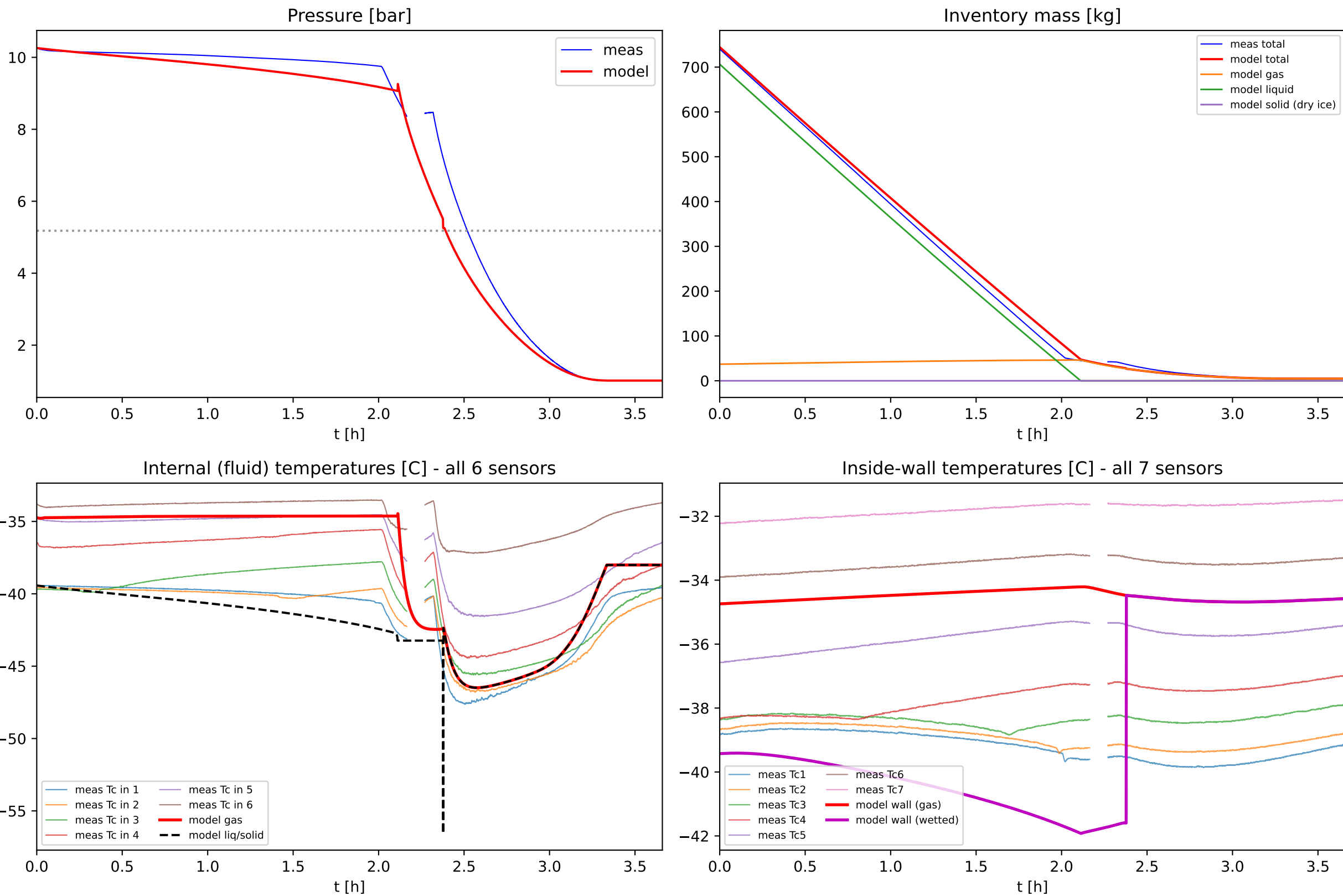
CARDICE Test 10 (liquid) - model vs 1 Hz data (all sensors)
