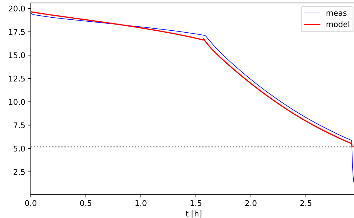
CARDICE Test 6 (liquid) - model vs 1 Hz data (all sensors)
