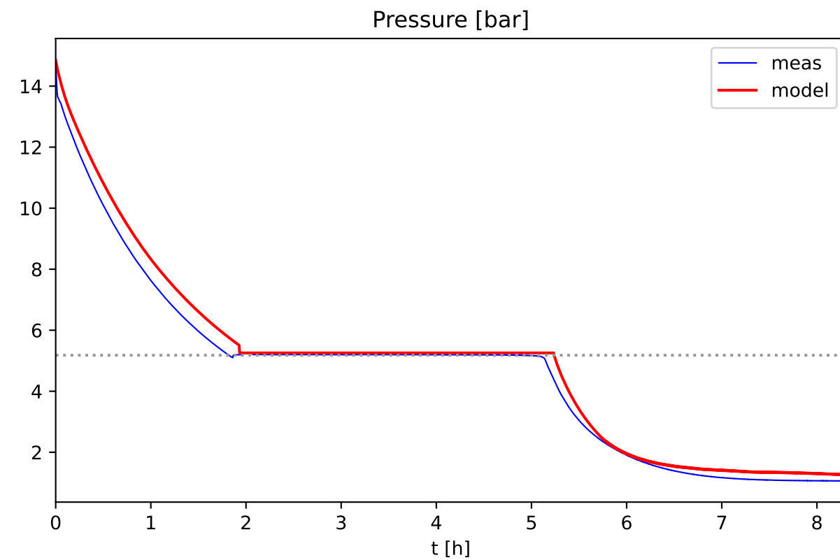
CARDICE Test 7 (gas) - model vs 1 Hz data (all sensors)
