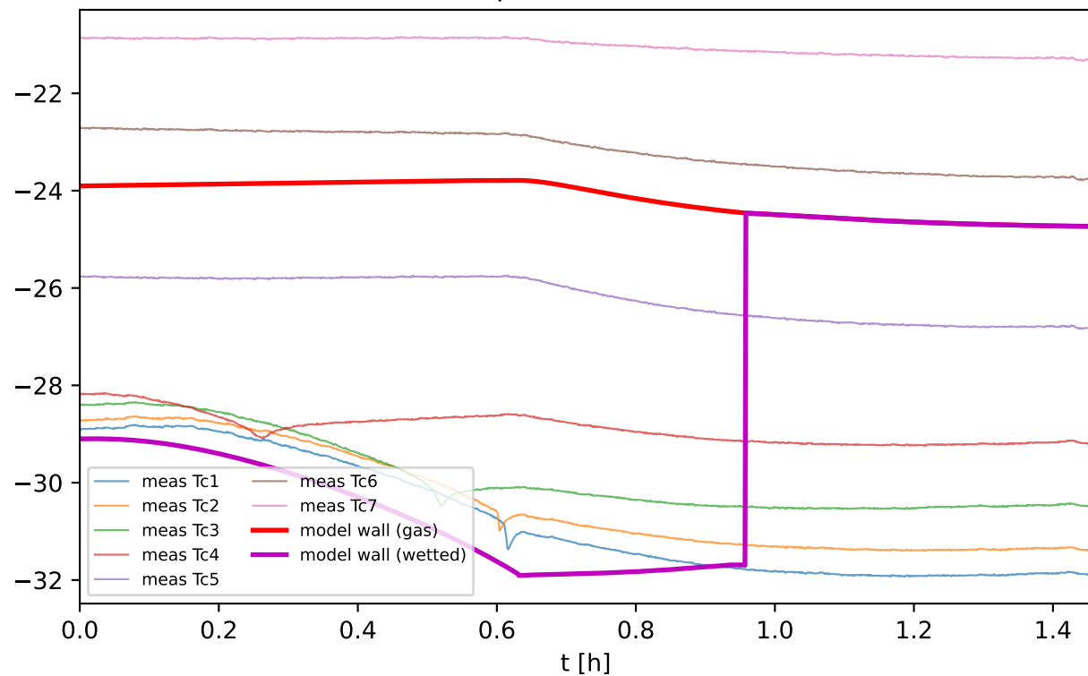
Inside-wall temperatures [C] - all 7 sensors
