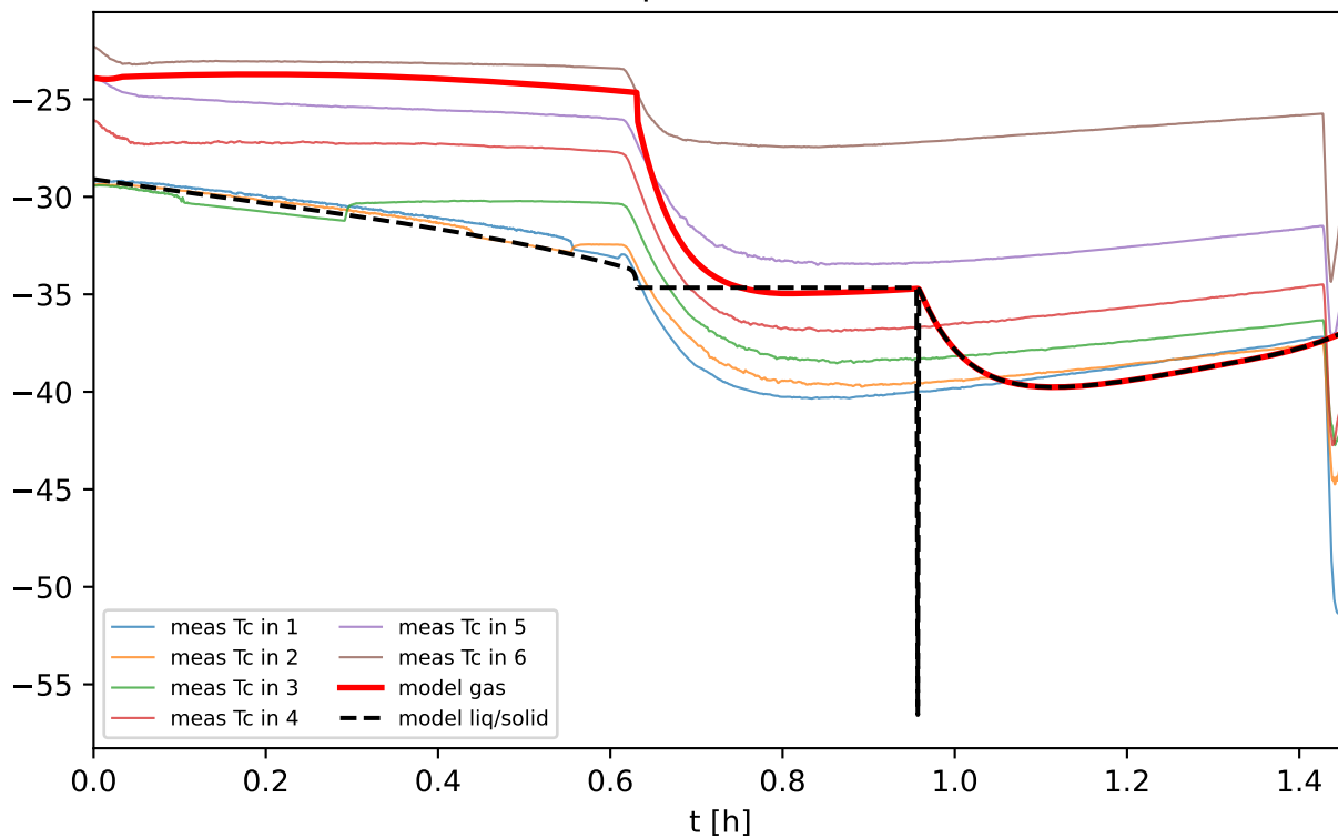
Internal (fluid) temperatures [C] - all 6 sensors
