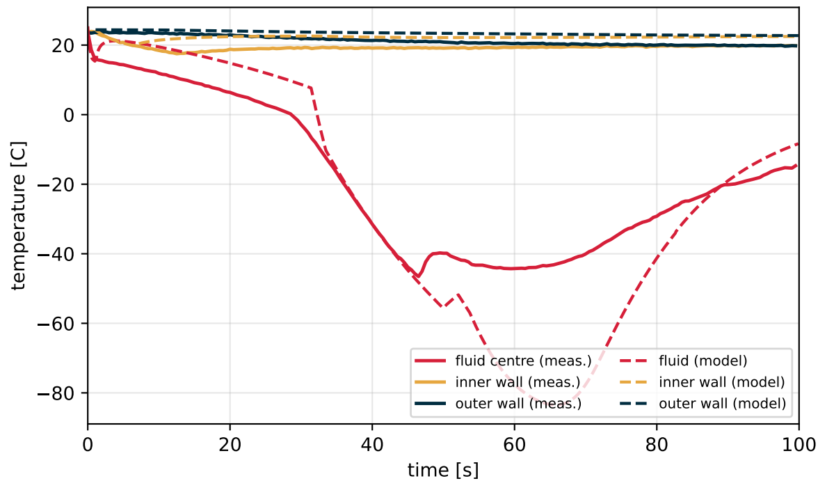
(c) z = 0.77 m
