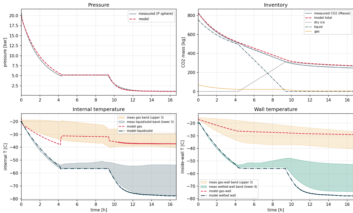
Fig. 8.1: Test 5 - gas release, 20 bar. Long triple-point plateau, ~ 266 kg retained dry ice, wetted wall to -78^{\circ}\text{C} .
