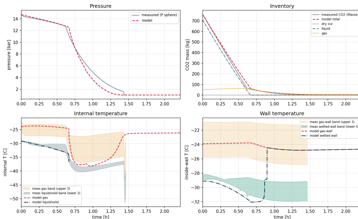
Fig. 8.4: Test 8 - liquid release, 15 bar.
