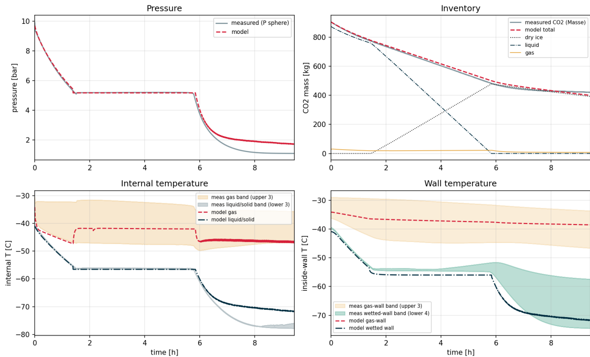
Fig. 8.5: Test 9 - gas release, 10 bar. The most retained dry ice ( \sim 392 kg).
