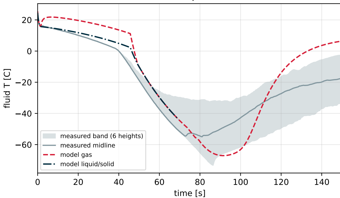
Fluid temperature
