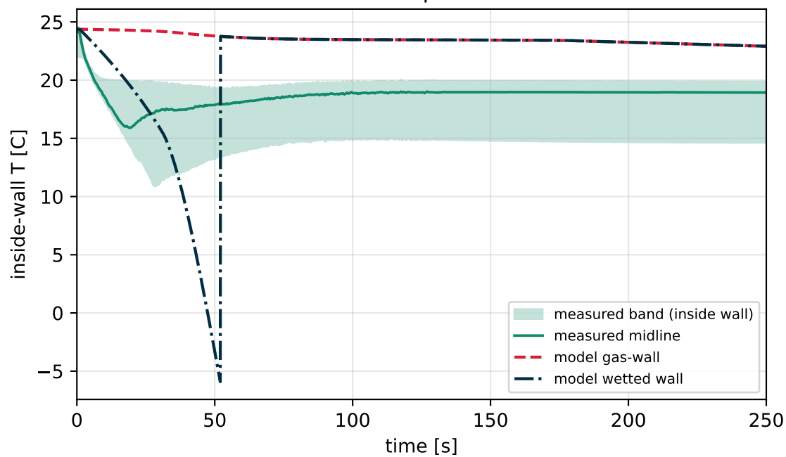
Wall temperature
