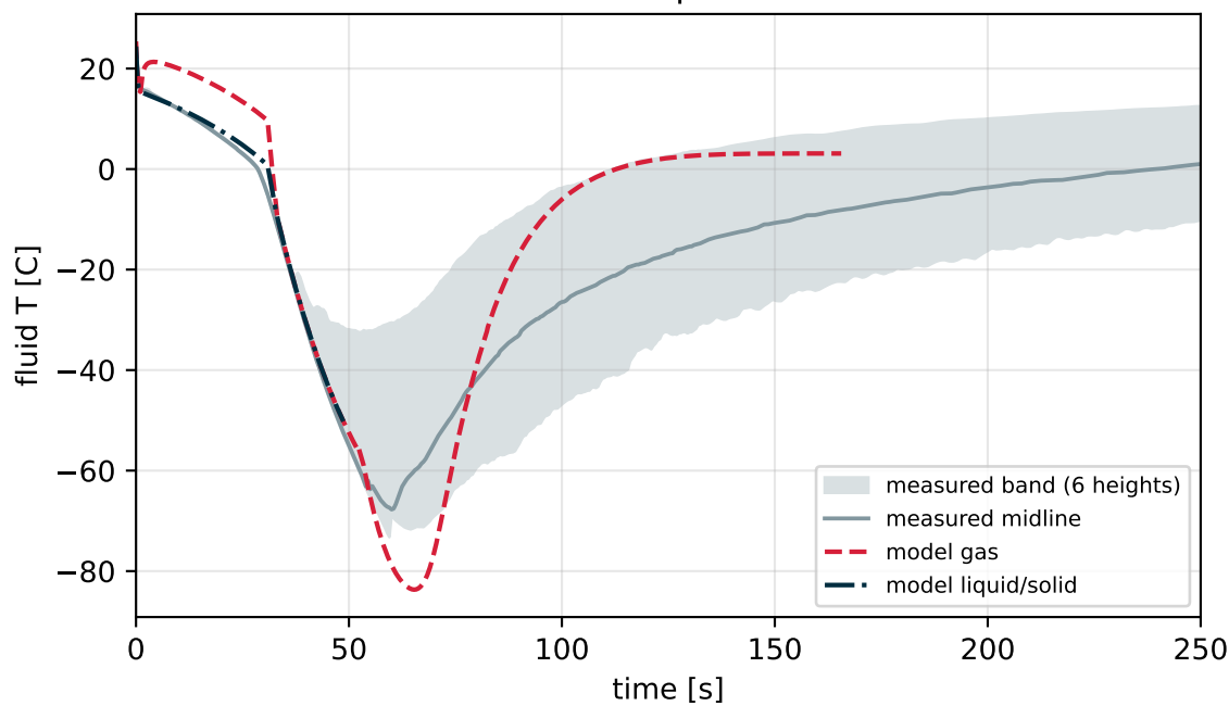
Fluid temperature
