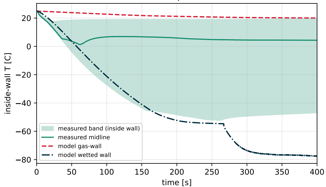
Wall temperature
