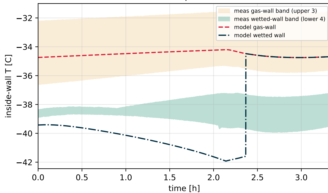
Wall temperature
